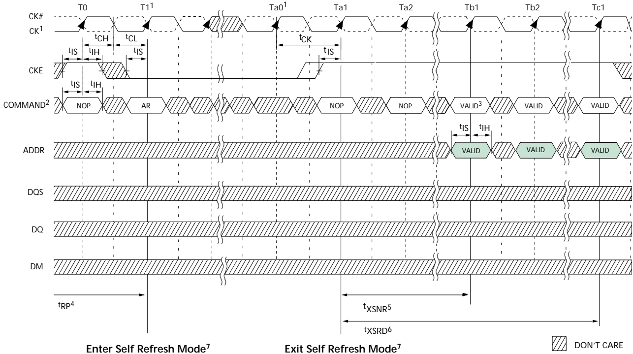
Figure 48: Self Refresh Mode
