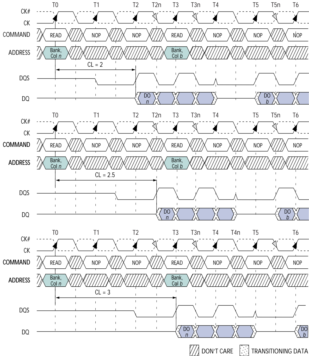
Figure 15: Nonconsecutive READ Bursts
