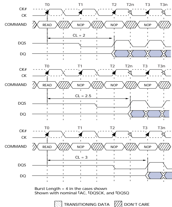
Figure 8: CAS Latency
