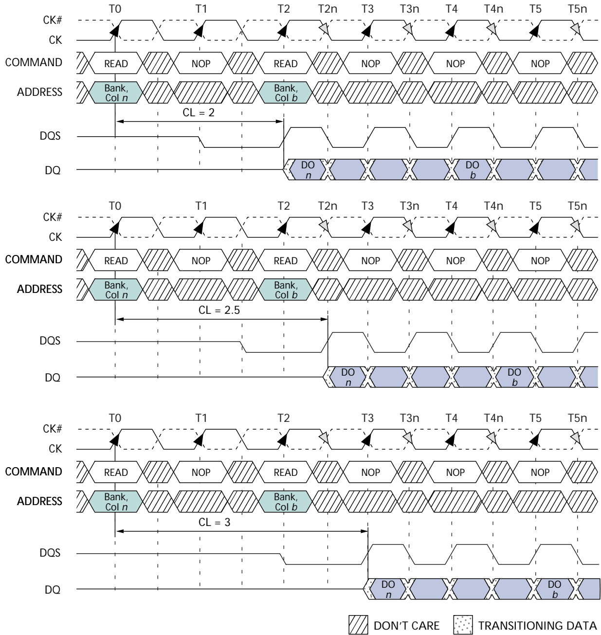
Figure 14: Consecutive READ Bursts
