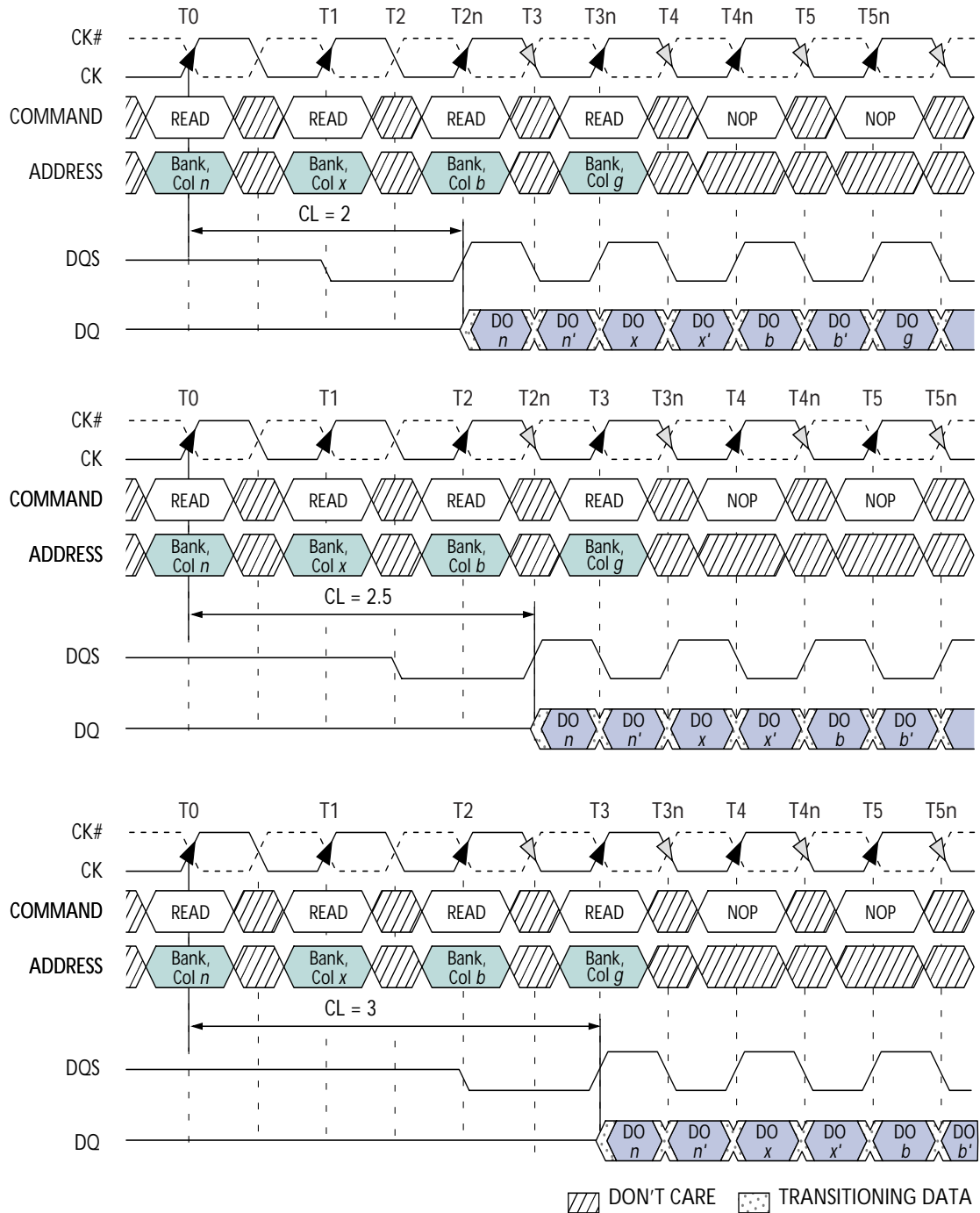
Figure 16: Random READ Accesses
