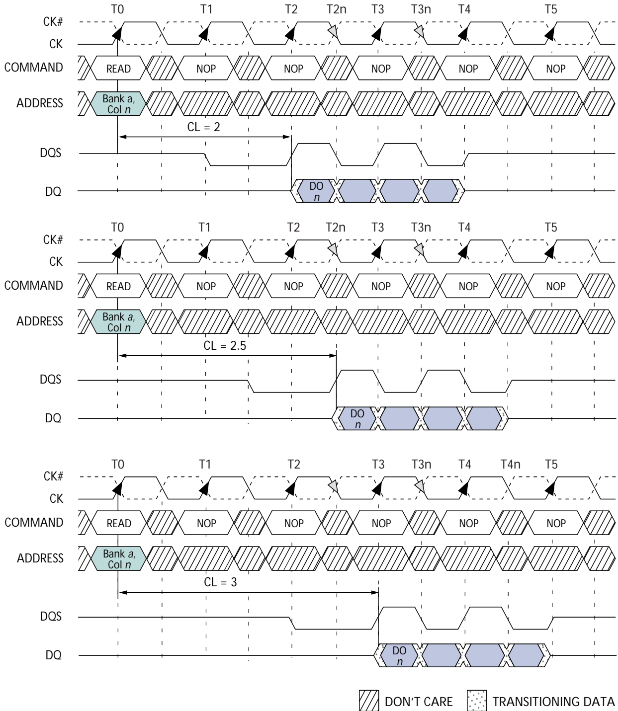
Figure 13: READ Burst
