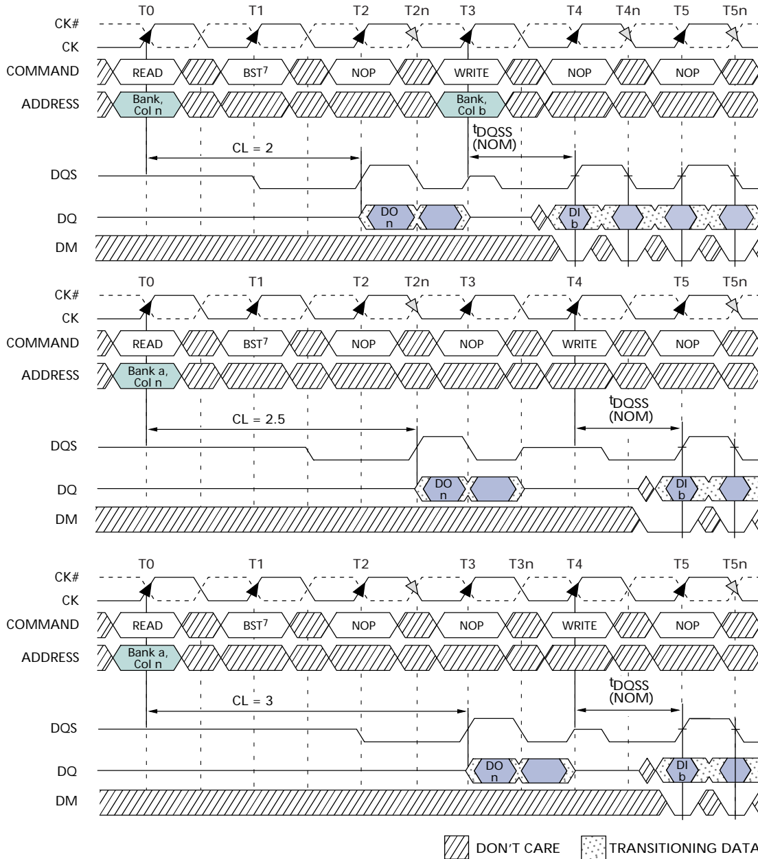
Figure 18: READ to WRITE
