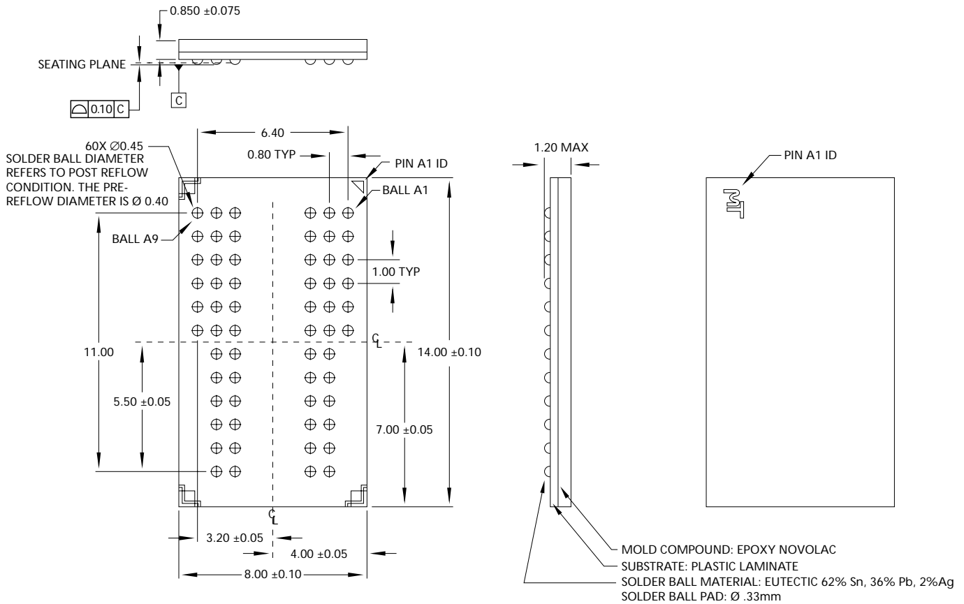
Figure 55: 60-Ball FBGA (8x14mm)
