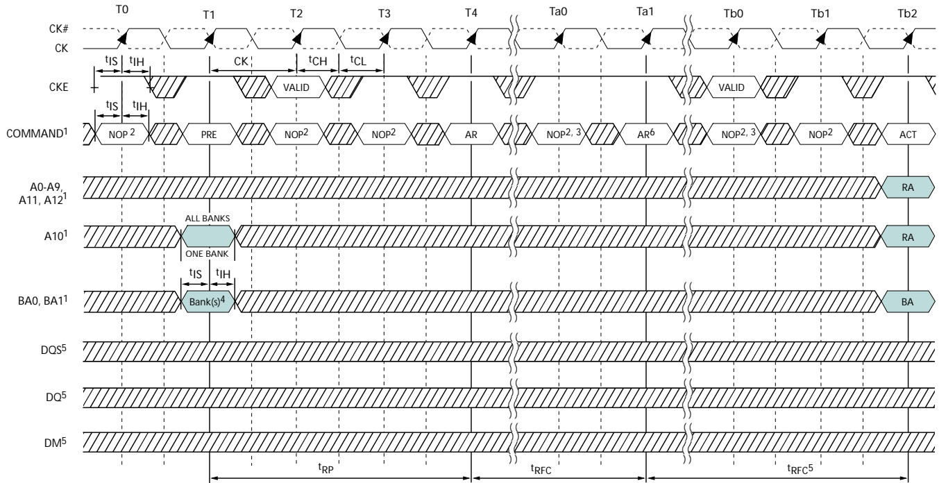
Figure 47: Auto Refresh Mode
